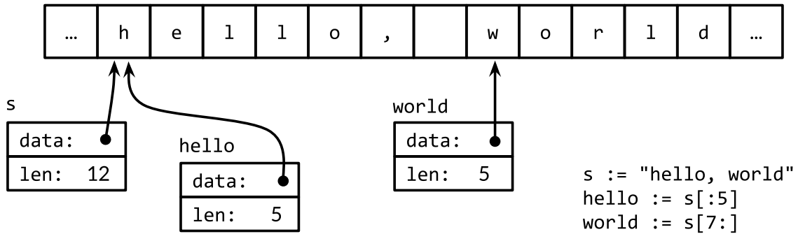
Figure 3.4. The string "hello, world" and two substrings.
