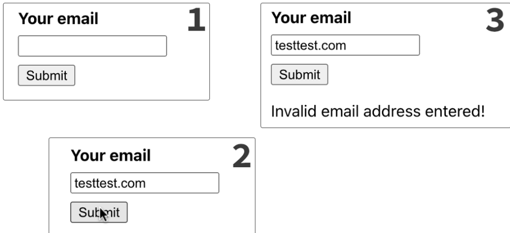
Figure 5.7: The final user interface of this activity
