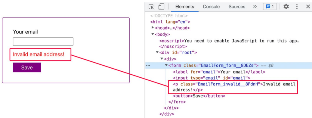
Figure 7.4: The error message DOM element sits right below the <input> it belongs to
