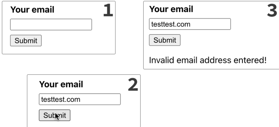
Figure 5.9: The final user interface of this activity
