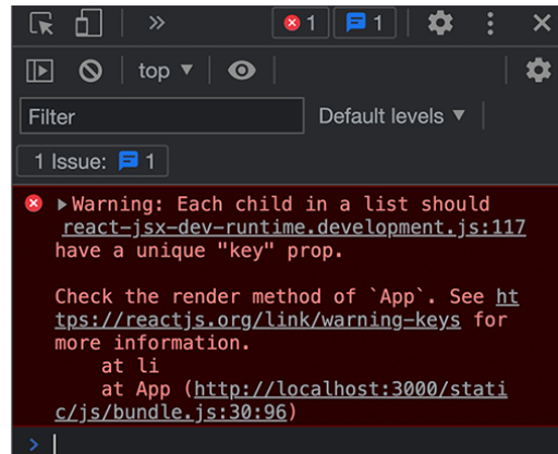
Figure 5.3: React sometimes generates a warning regarding missing unique keys
