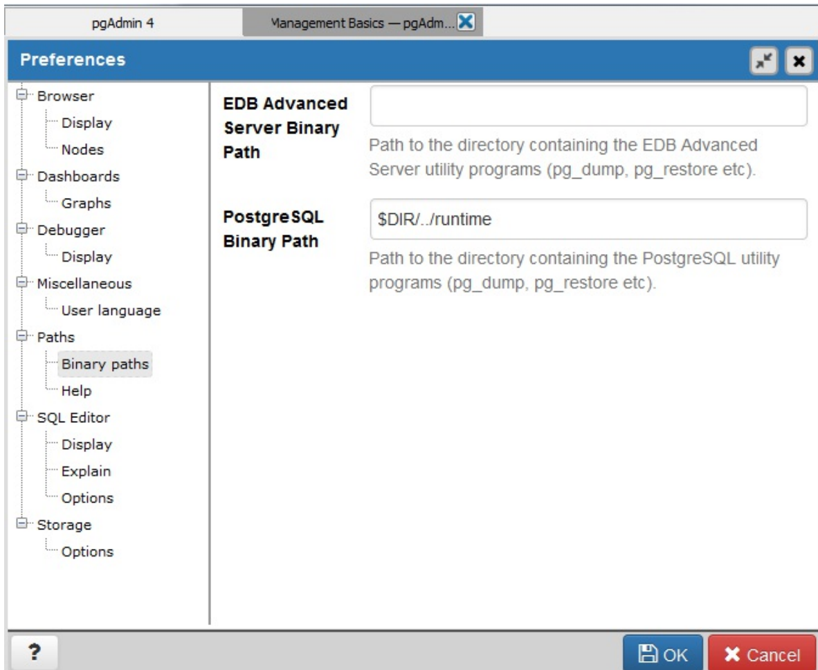
Figure 4-13. pgAdmin File→Preferences
