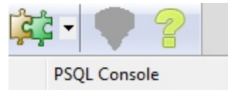
Figure 4-4. psql plugin
