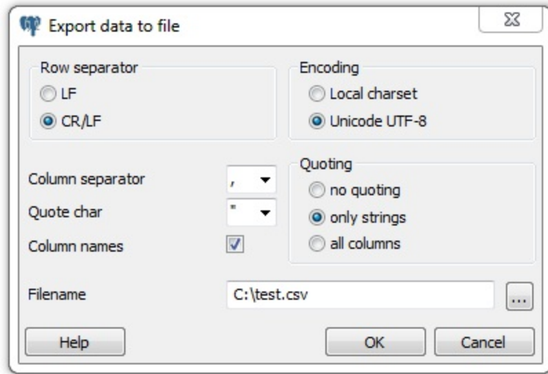
Figure 4-11. Export menu
