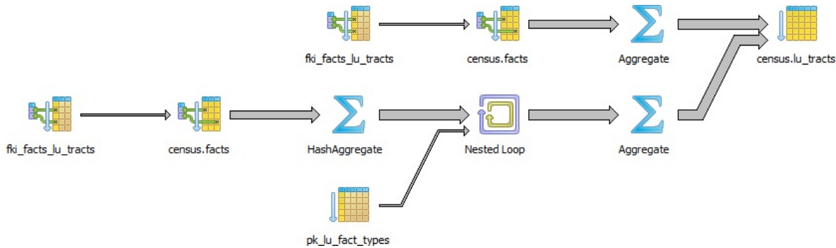
Figure 9-4. Graphical plan when overusing subqueries
