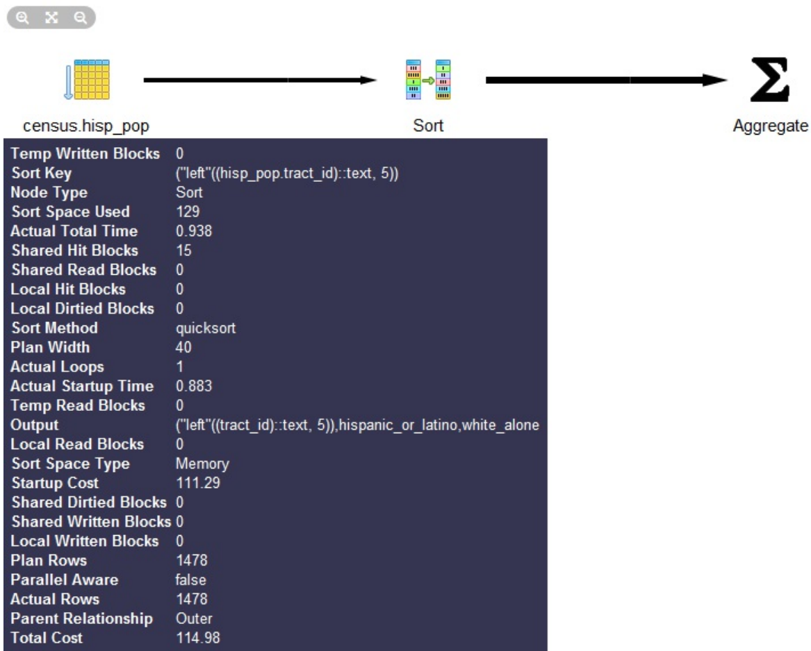
Figure 4-17. Graphical explain example
