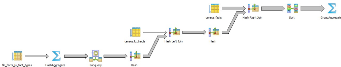
Figure 9-7. Graphical plan when using subqueries instead of CASE
