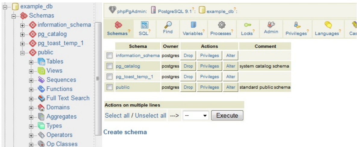
Figure 1-2. phpPgAdmin
