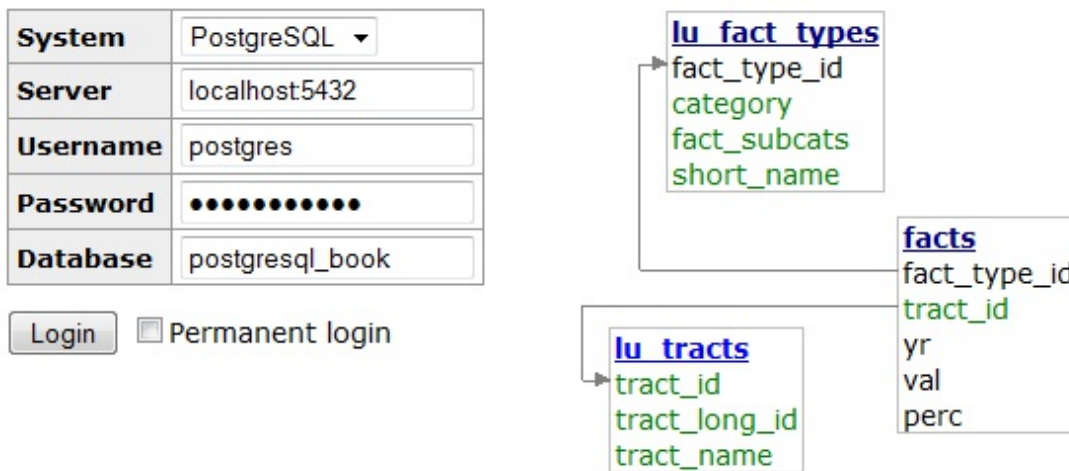
Figure 1-3. Adminer
