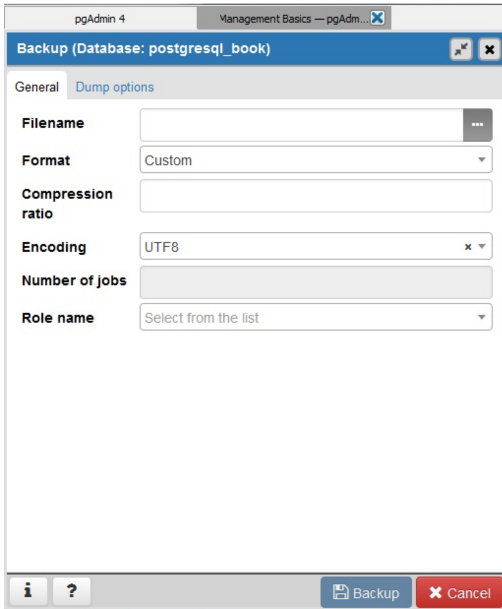
Figure 4-14. Backup database
