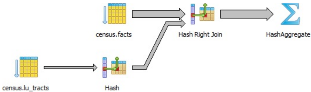
Figure 9-8. Graphical explain when using CASE
