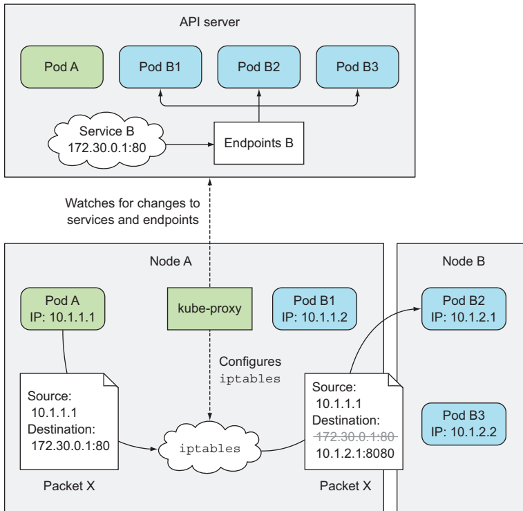
Figure 11.17 Network packets sent to a Service’s virtual IP/port pair are modified and redirected to a randomly selected backend pod.
