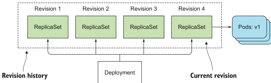
Figure 9.11 A Deployment's ReplicaSets also act as its revision history.
