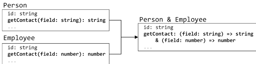
Figure 10.11 Merging methods
