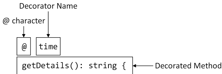
Figure 14.1 Applying a method decorator
