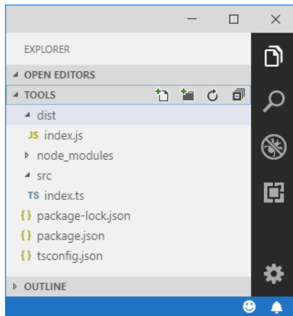
Figure 5.1 The contents of the example project folder
