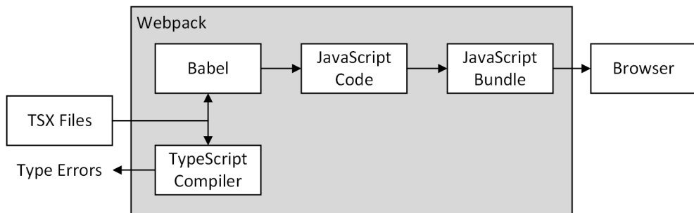
Figure 20.3 The TypeScript React development toolchain.
