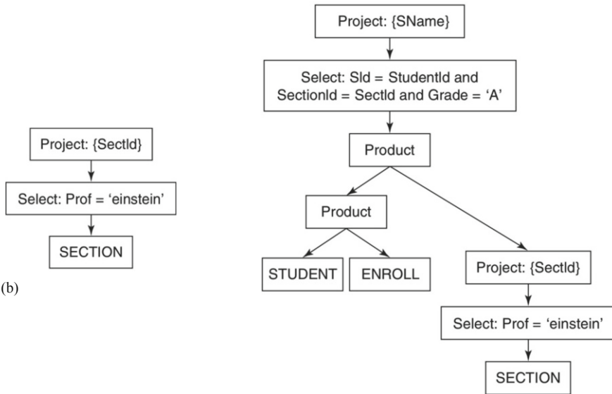
Fig. 10.12 Applying the basic query planning algorithm in the presence of views. (a) The SQL query, (b) the tree for the view, (c) the tree for the entire query
