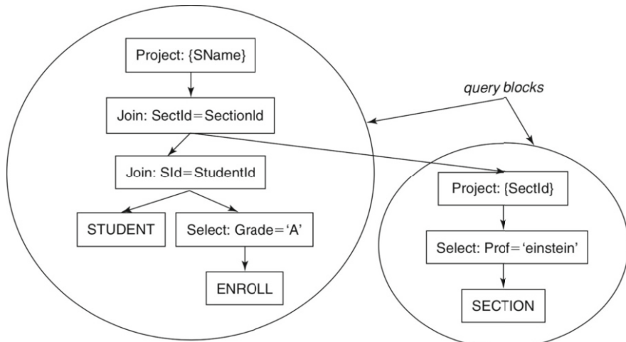
Fig. 15.20 Planning a view query. (a) A view definition and a query that uses it, (b) planning each query block separately
