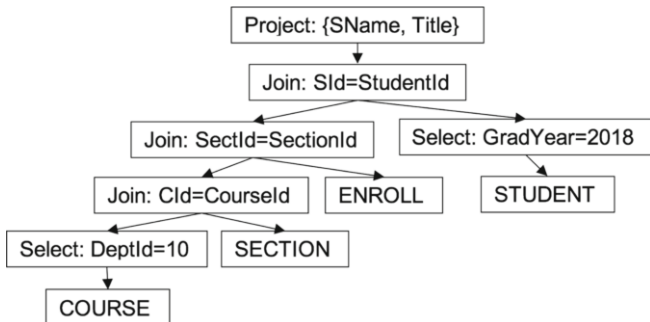
Fig. 15.12 Equivalent query trees having different skeletons. (a) The SQL query, (b) a left-deep query tree, (c) another left-deep query tree, (d) yet another left-deep query tree, (e) a right-deep query tree, (f) a bushy query tree
