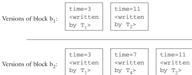
Fig. 5.24 Multiversion concurrency
