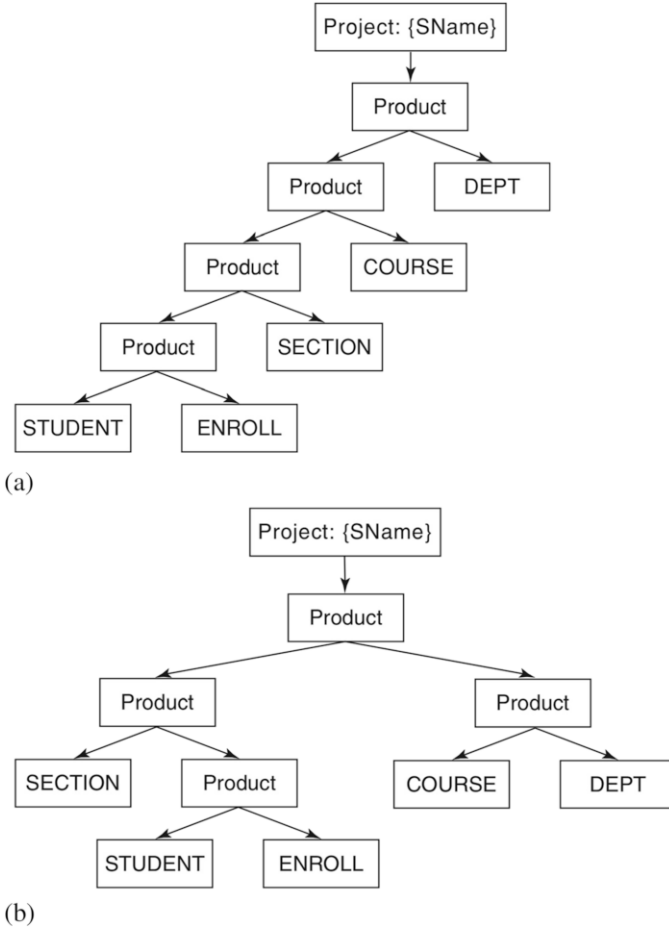
Fig. 15.2 Rearranging product nodes to produce an equivalent query tree. (a) A tree produced by the basic planner, (b) the result of applying associative and commutative transformations
