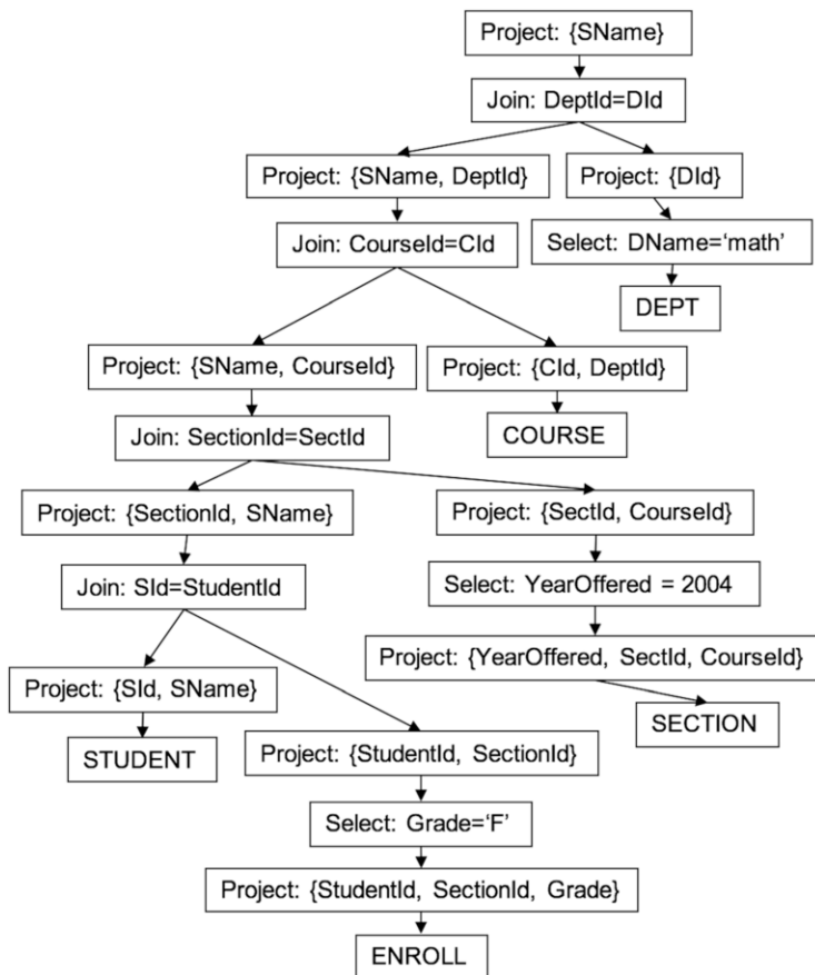
Fig. 15.8 Adding projections to the query tree of Fig. 15.7
