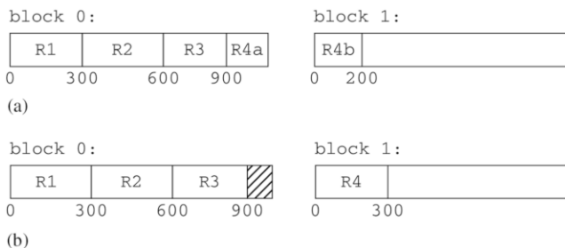
Fig. 6.1 Spanned versus unspanned records. (a) Record R4 spans blocks 0 and 1, (b) record R4 is stored entirely in block 1
