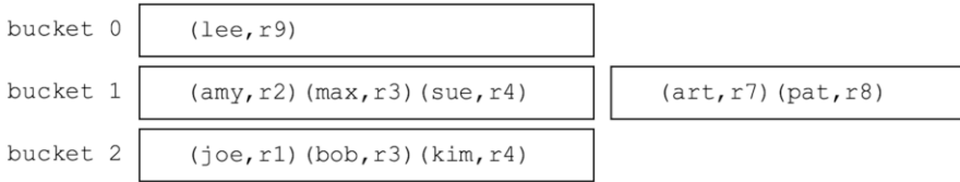
Fig. 12.5 A static hash index with three buckets
