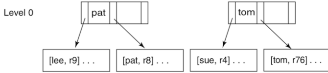
Fig. 12.17 Splitting a directory block
