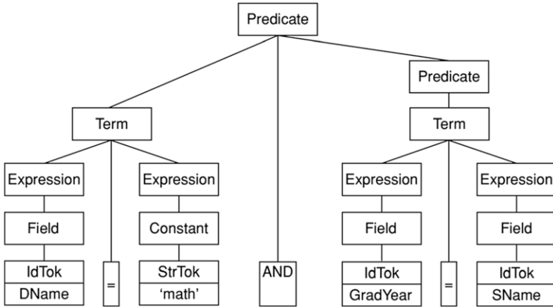
Fig. 9.6 A parse tree for the string DName = 'math' AND GradYear = SName
